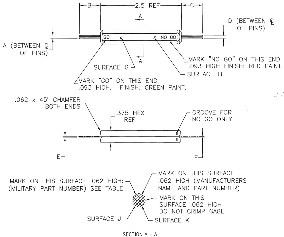
FIGURE 1 – AS22520/18 GAGE CONFIGURATION
