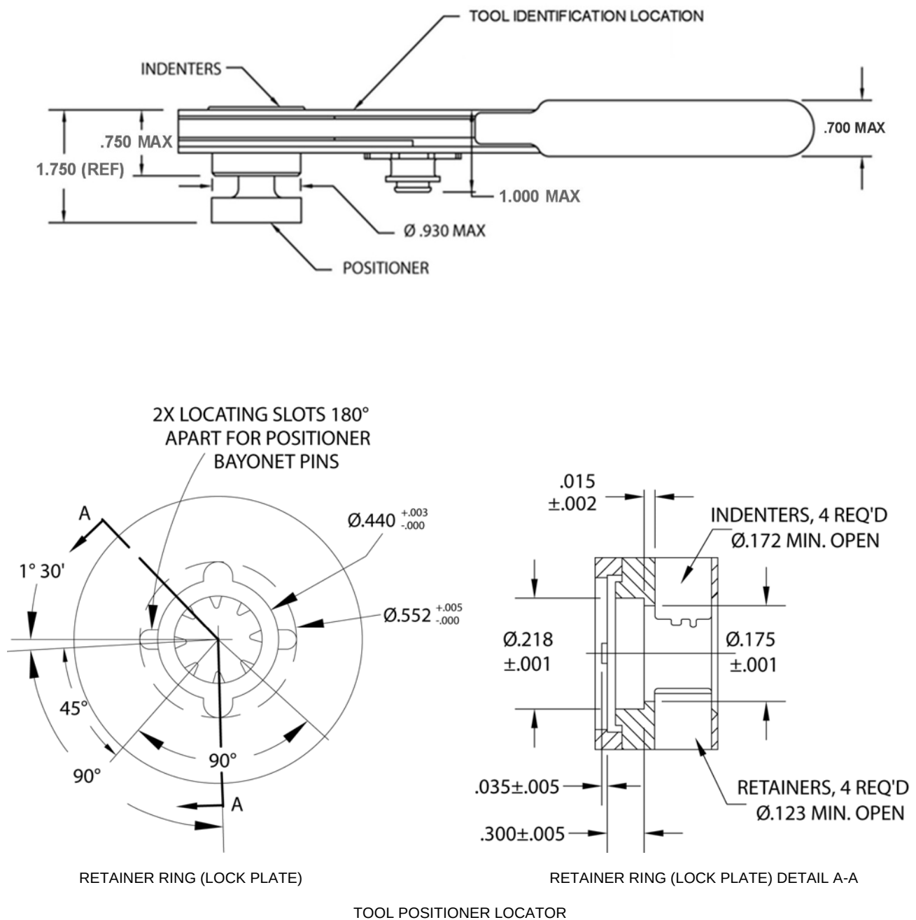
FIGURE 1 - M22520/19-01 TOOL (CONTINUED)
