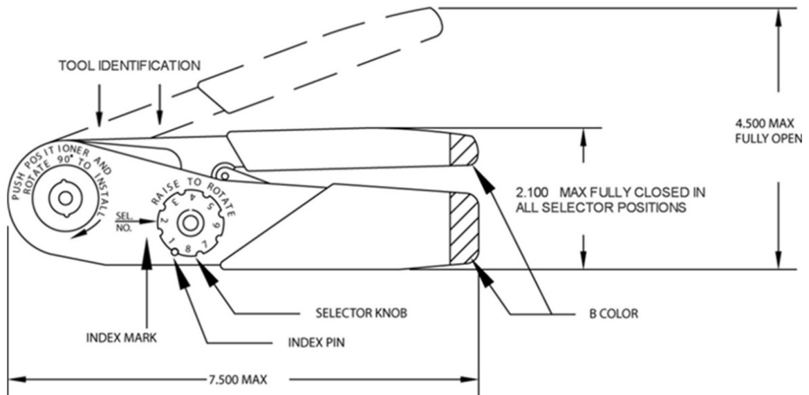
FIGURE 1 - M22520/19-01 TOOL
