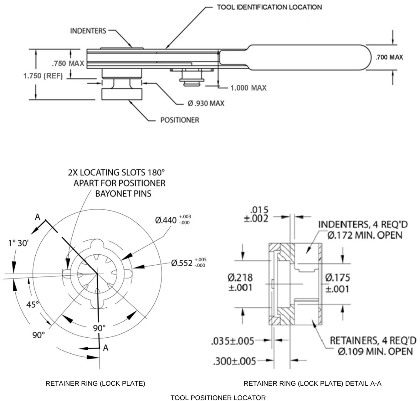
FIGURE 1 - M22520/20-01 TOOL (CONTINUED)
