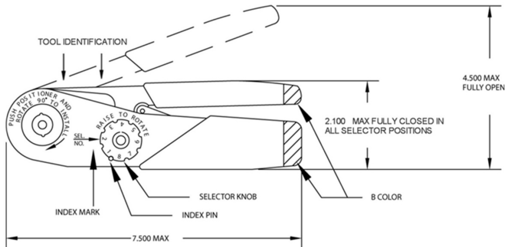
FIGURE 1 - M22520/20-01 TOOL
