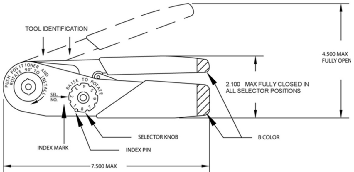
FIGURE 1 - M22520/21-01 TOOL
