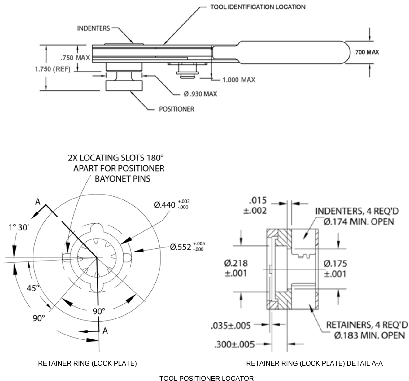
FIGURE 1 - M22520/21-01 TOOL (CONTINUED)
