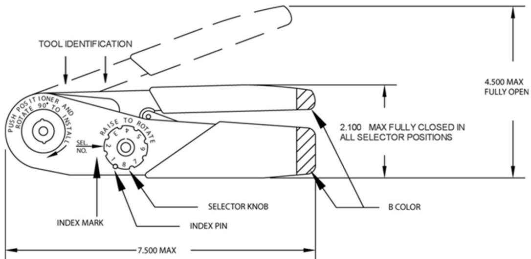
FIGURE 1 - M22520/22-01 TOOL
