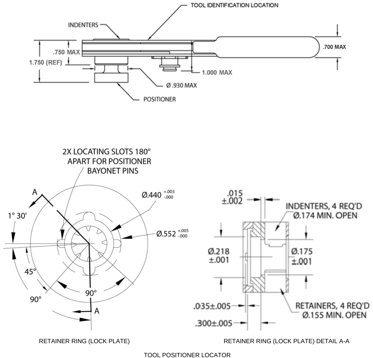
FIGURE 1 - M22520/22-01 TOOL (CONTINUED)
