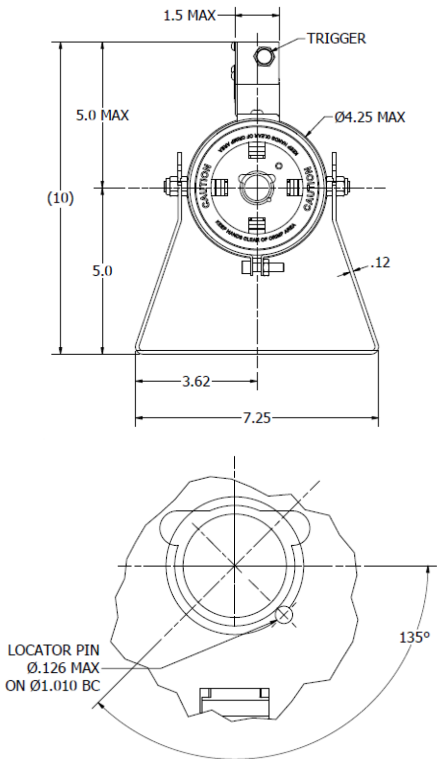
FIGURE 1 - M22520/23-01 BASIC TOOL (CONT.)
