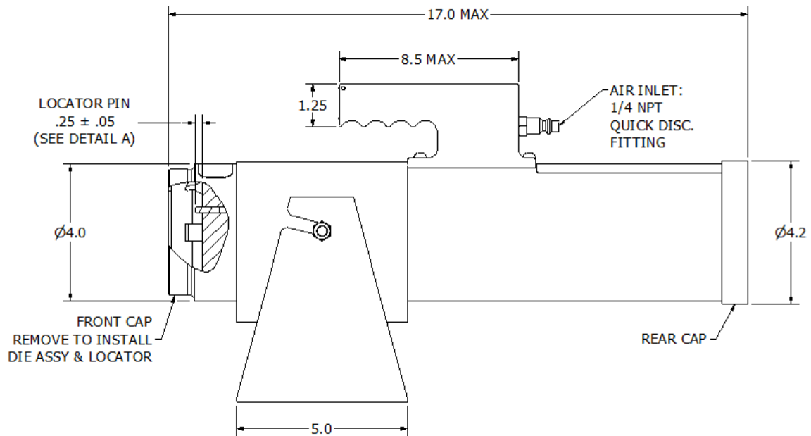
SIDE VIEW
