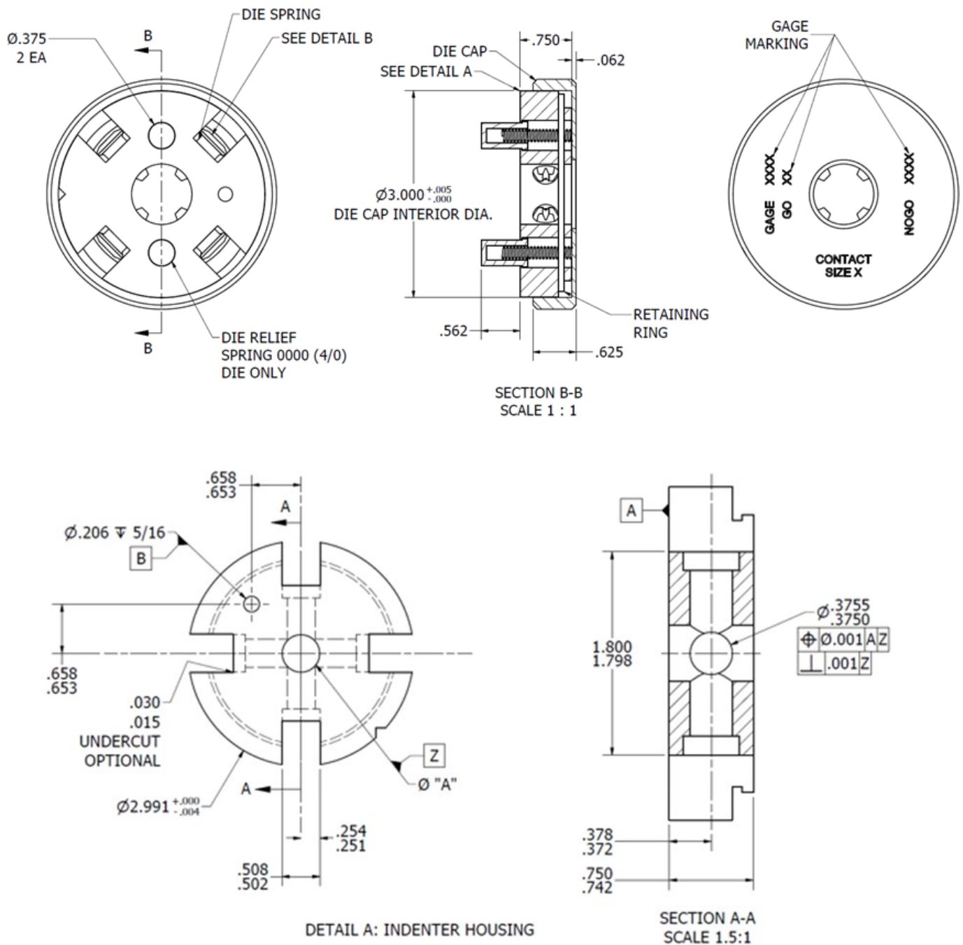
FIGURE 2 - DIE CAP AND DIE ASSEMBLY
