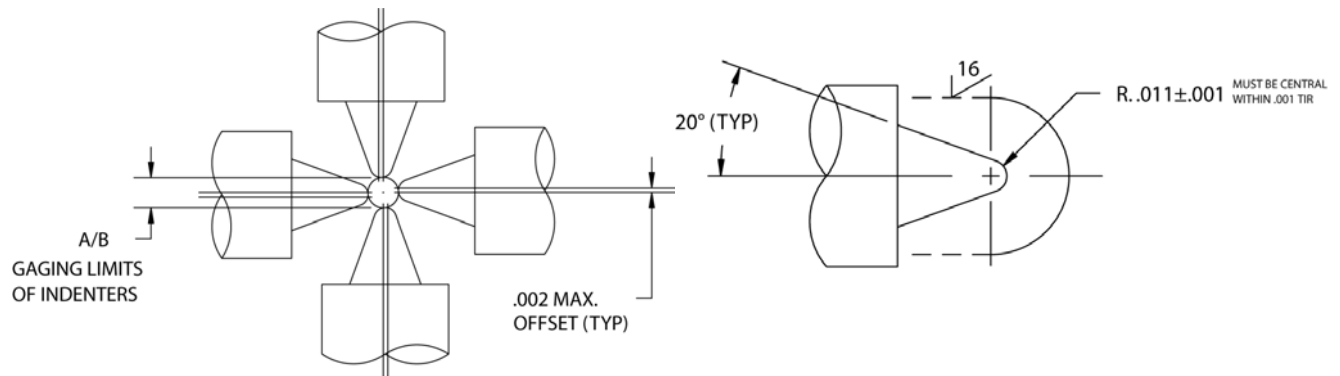
INDENTER LOCATIONS WITH TOOL IN FULLY CLOSED POSITION
