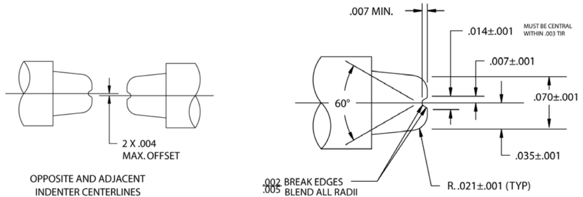
INDENTERS
