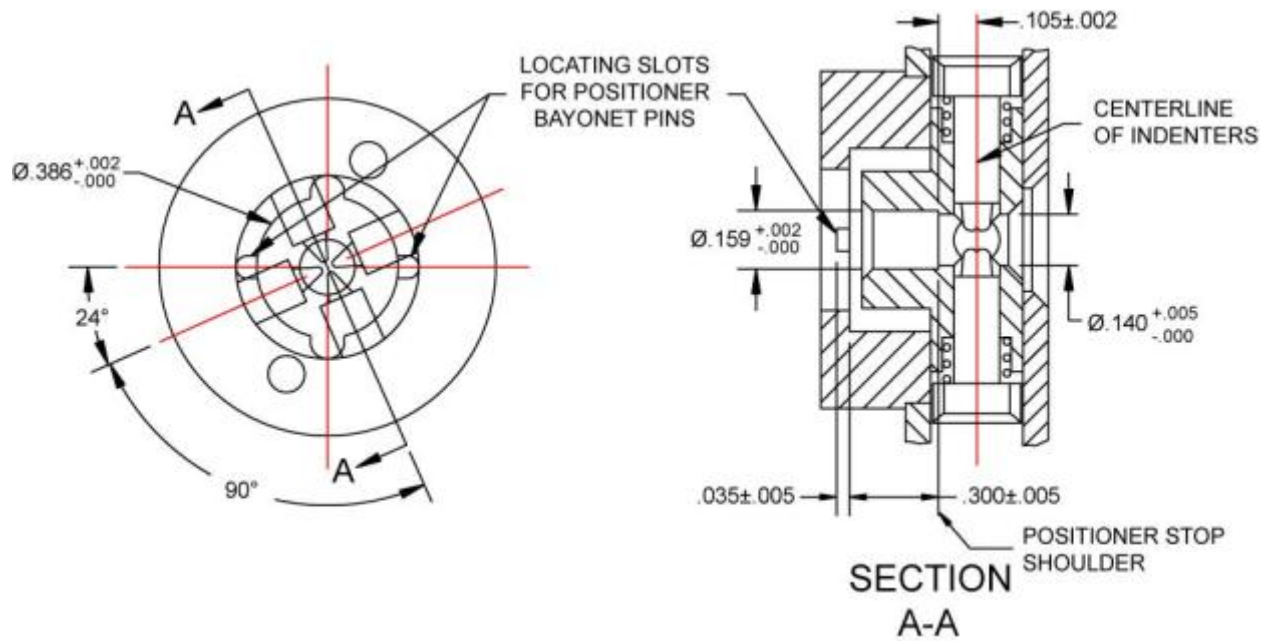
RETAINER RING
