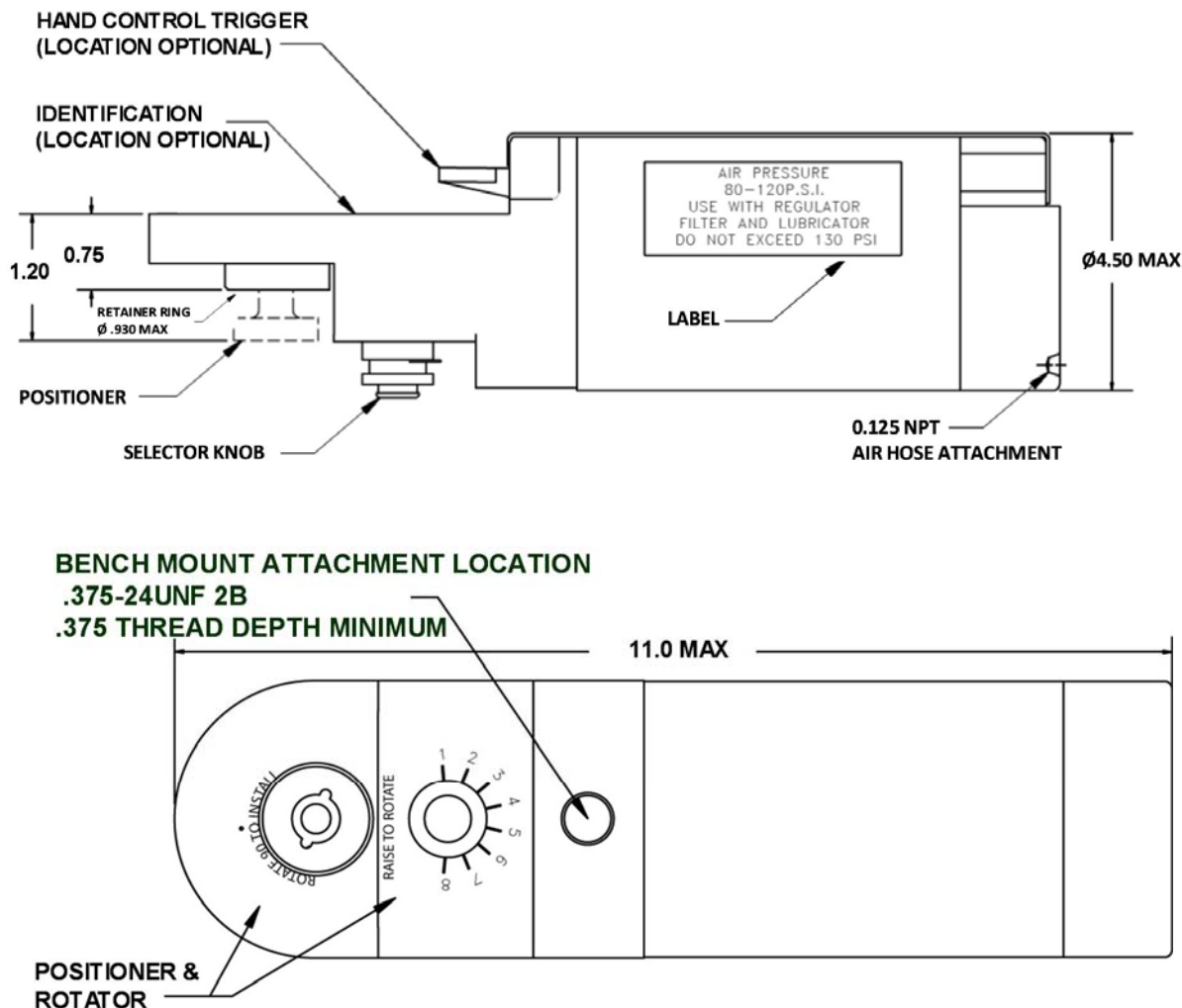
FIGURE 1 - M22520/28-01 PNEUMATIC CRIMP TOOL FRAME
