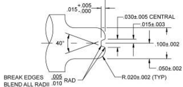
FIGURE 2 - M22520/29-01 RETAINER RING AND INDENTERS
