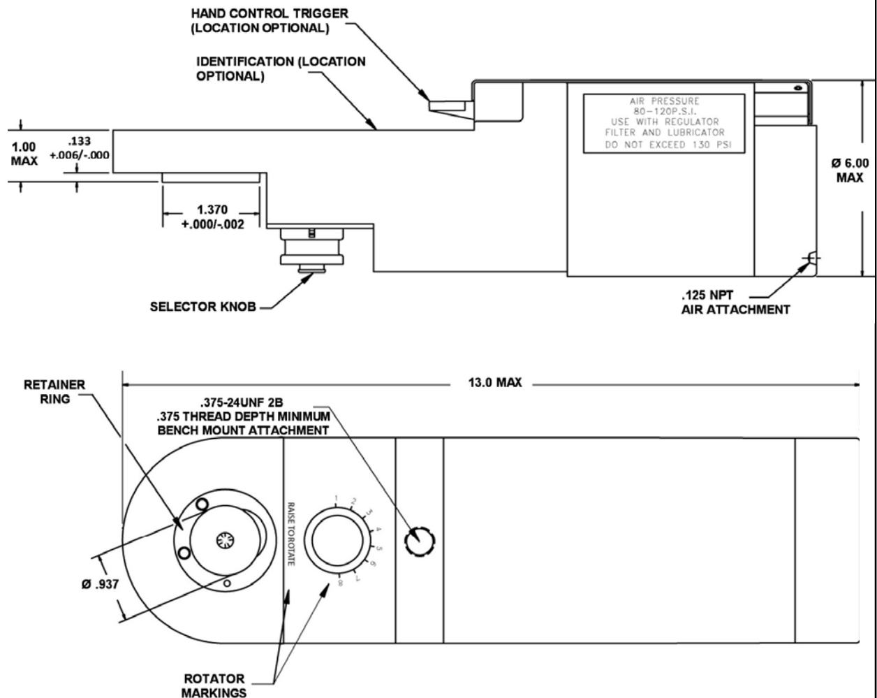
FIGURE 1 - M22520/29-01 PNEUMATIC CRIMP TOOL
