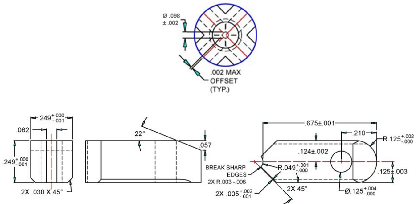
DETAIL B - INDENTER DETAILS WITH TOOL IN FULLY CLOSED POSITION
