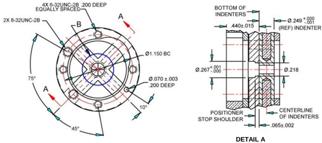
RETAINER RING DETAILS
