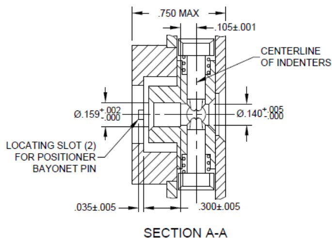
M22520/34-01 POSITIONER LOCK PLATE (RETAINER RING) DETAILS
