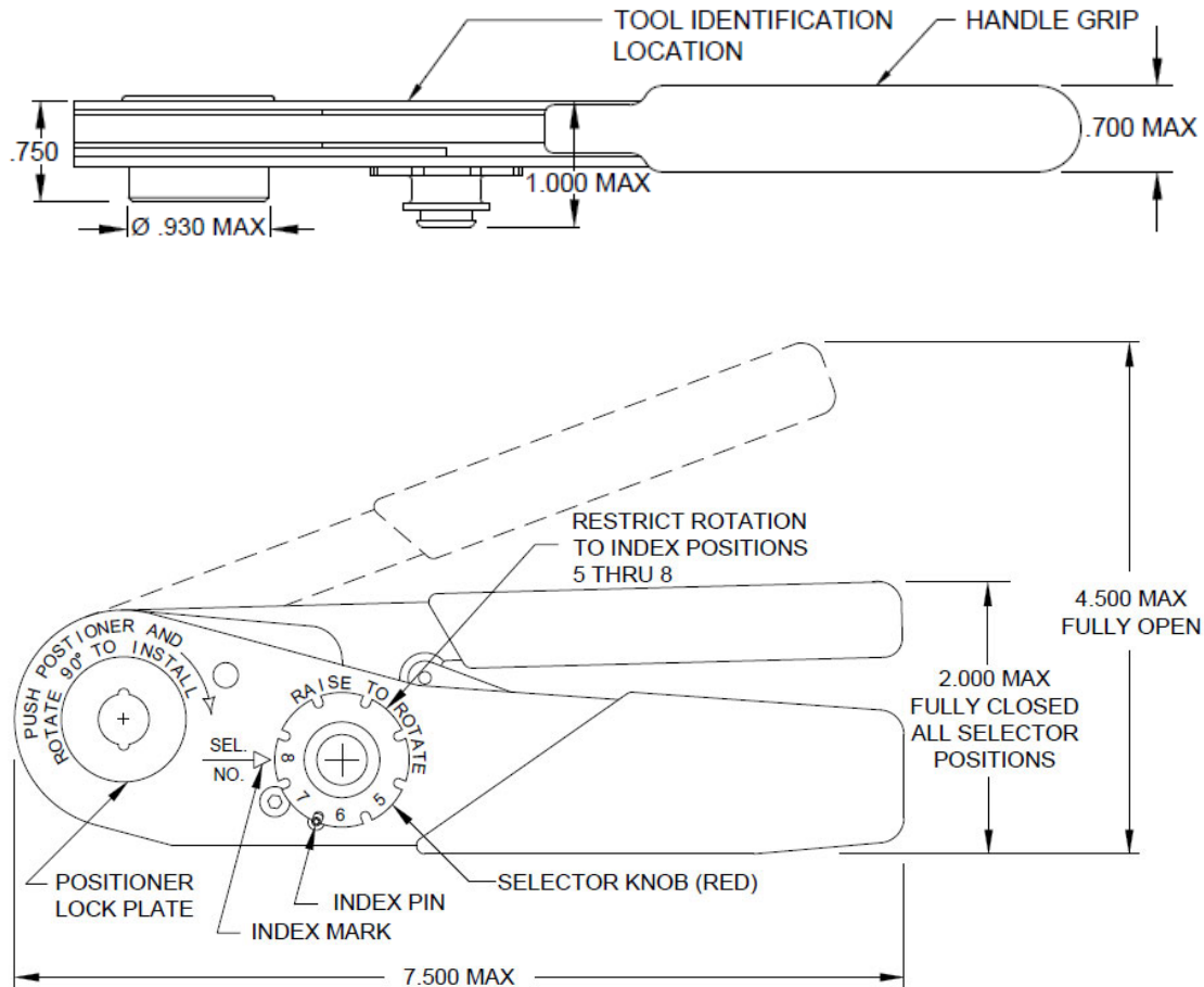
FIGURE 1 - M22520/34-01 TOOL
