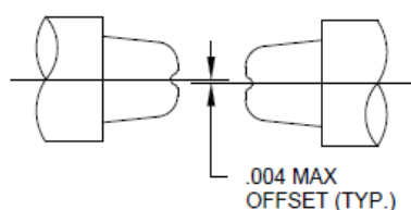
OPPOSITE AND ADJACENT INDENTER CENTERLINES
