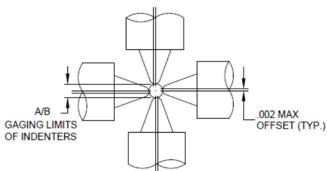
INDENTER LOCATIONS WITH TOOL IN FULLY CLOSED POSITION
