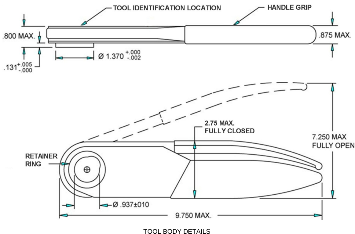
FIGURE 1 - AS22520/4-01 BASIC TOOL
