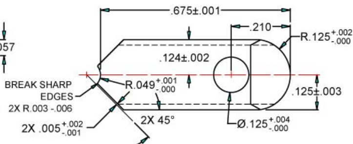
DETAIL B - INDENTER DETAILS WITH THE TOOL IN THE FULLY CLOSED POSITION
