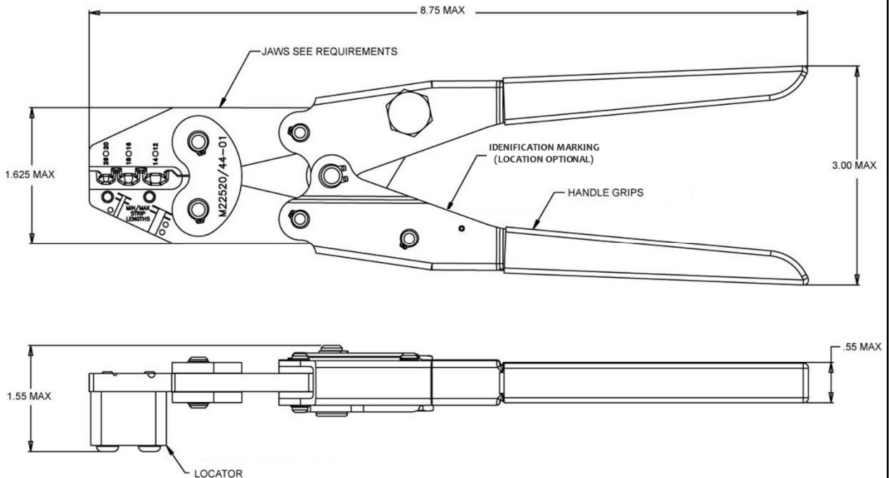
FIGURE 1 - M22520/44-01 CRIMPING TOOL
