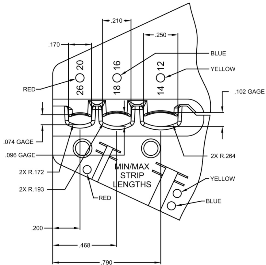
FIGURE 2 - M22520/44-01 CRIMPING TOOL JAW DETAIL
