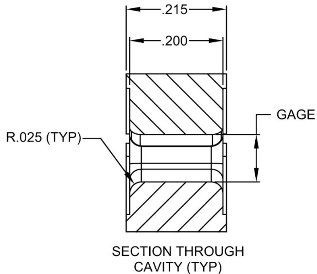
FIGURE 3 - M22520/44-01 CRIMP CAVITY SECTION, TYPICAL
