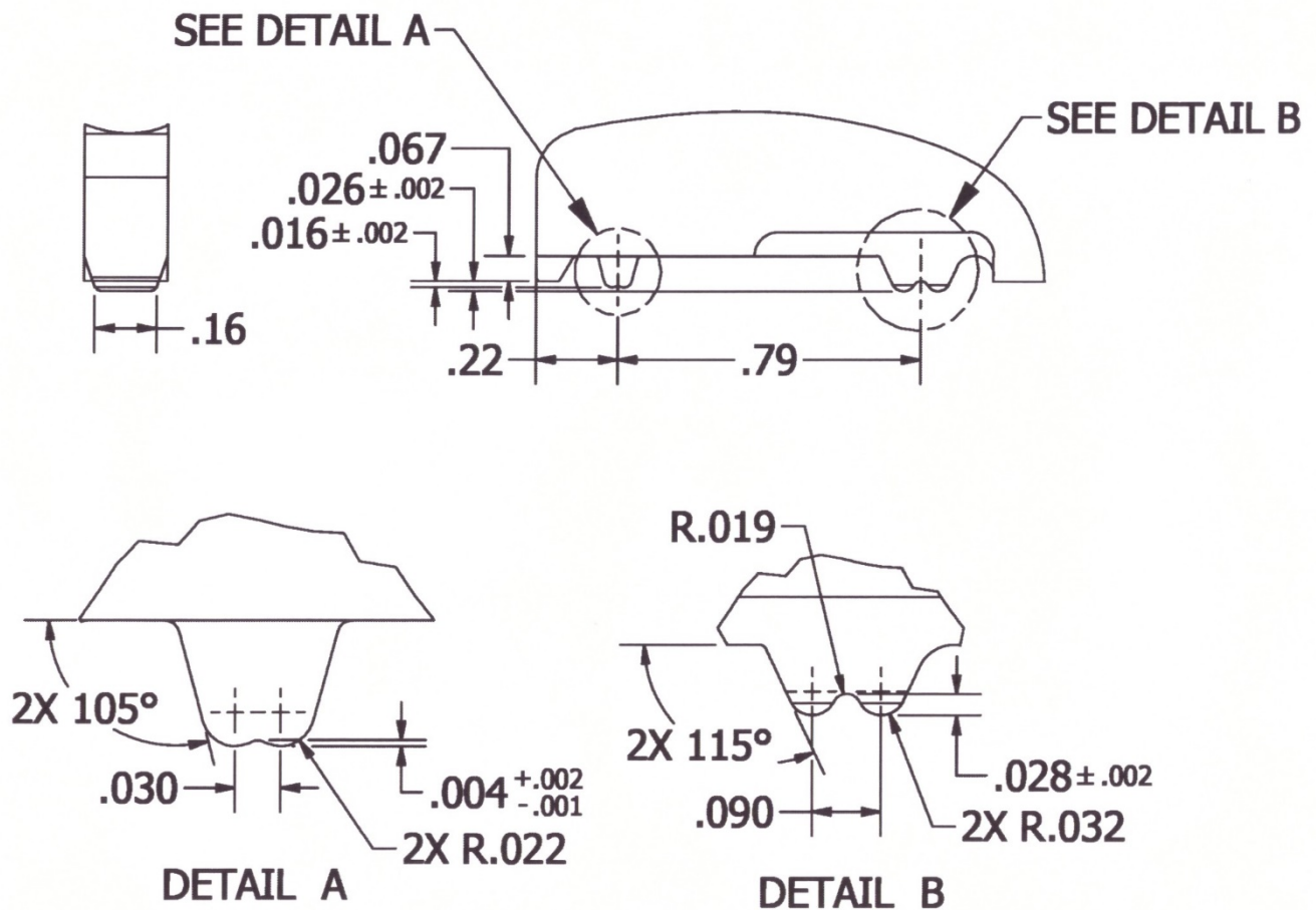
FIGURE 3 - UPPER DIE FOR TOOL FRAME JAWS (SEE REQUIREMENT 1)
