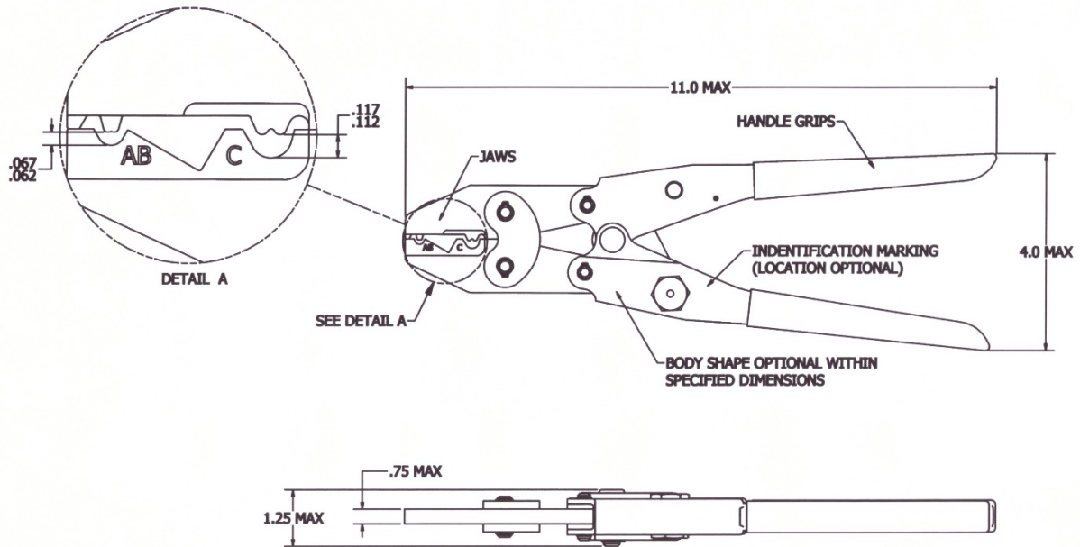
FIGURE 1 - TOOL FRAME
