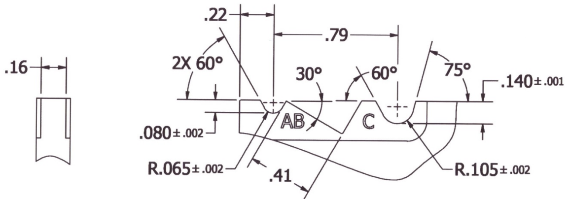
FIGURE 2 - LOWER DIE FOR TOOL FRAME JAWS (SEE REQUIREMENT 1)
