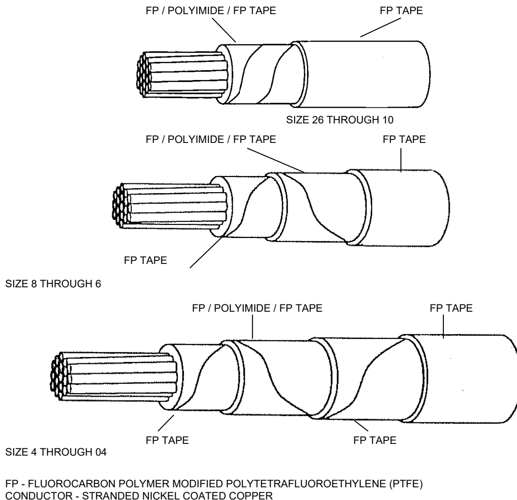
FIGURE 1 - AS22759/187 CONFIGURATION
