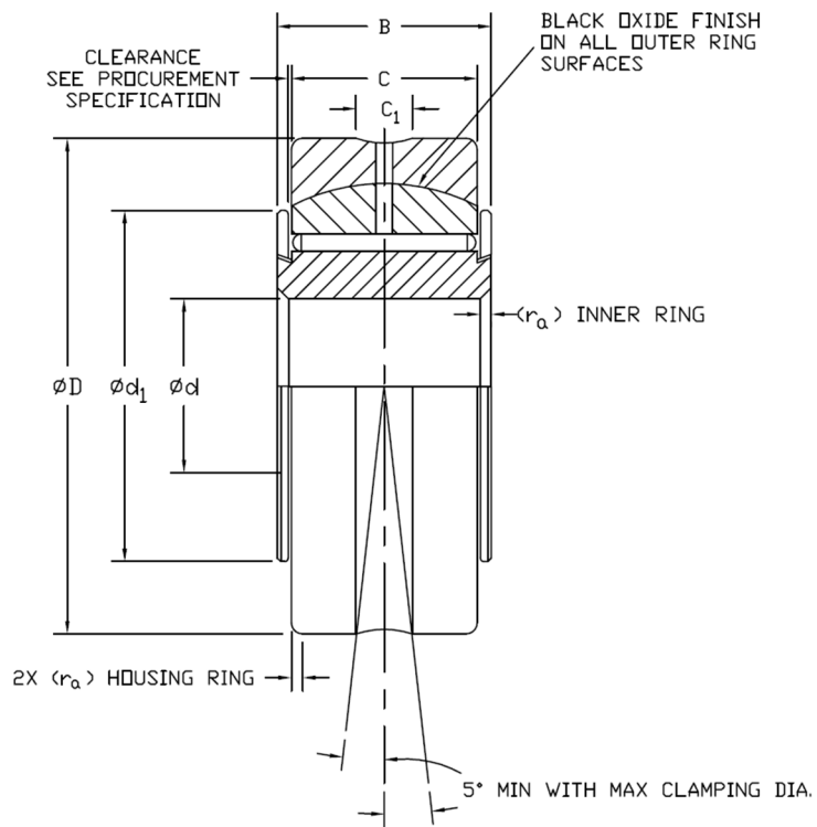
FIGURE 1 - PART CONFIGURATION
