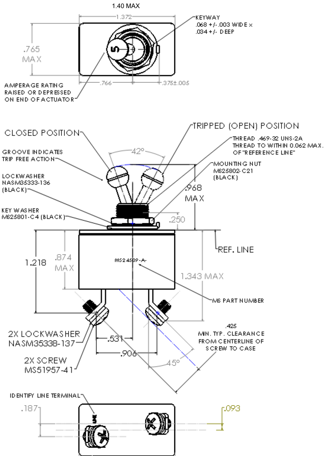
FIGURE 1 - CIRCUIT BREAKER (CONFIGURATION A-BUSHING MOUNT)
