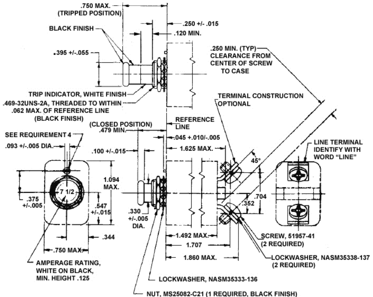
FIGURE 1 - CIRCUIT BREAKER CONFIGURATION AND DIMENSIONS
