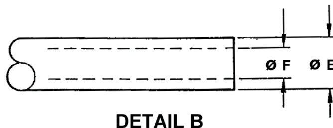
AS25486 CONTACT CRIMP BARREL (SEE TABLE 3) DASH -16 THRU -19 AND -30 THRU -33
