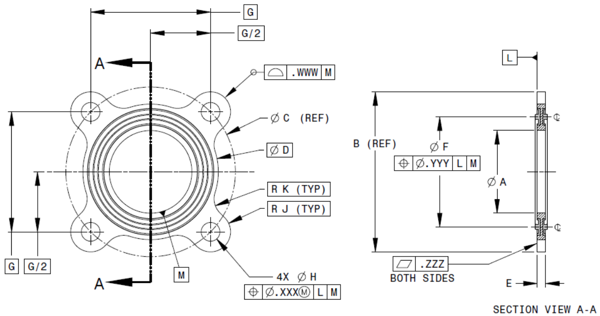
FIGURE 1 - SEAL -12 THRU -32
