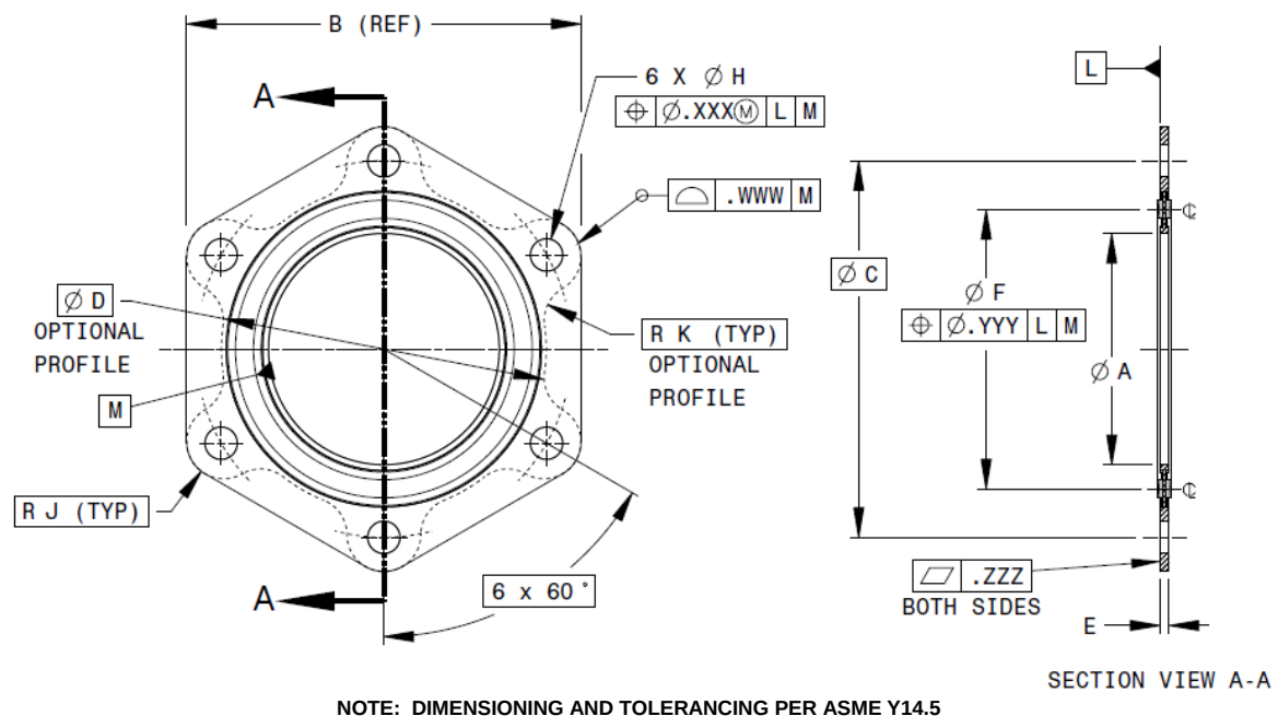
FIGURE 2 - SEAL -40 THRU -48
