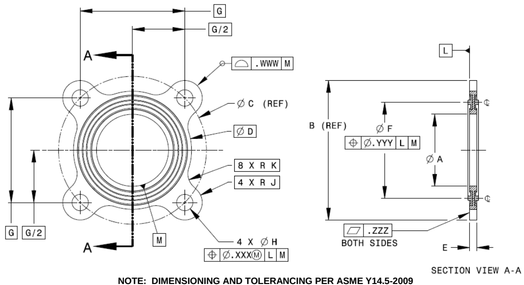
FIGURE 1 - SEAL -12 THRU -32
