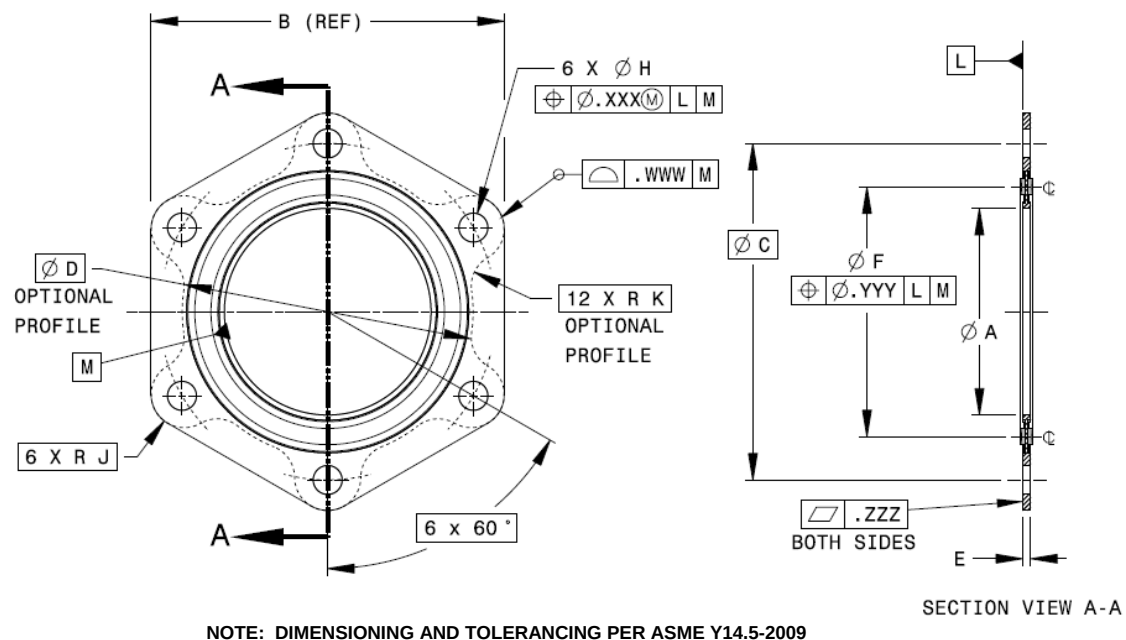
FIGURE 2 - SEAL -40 THRU -48
