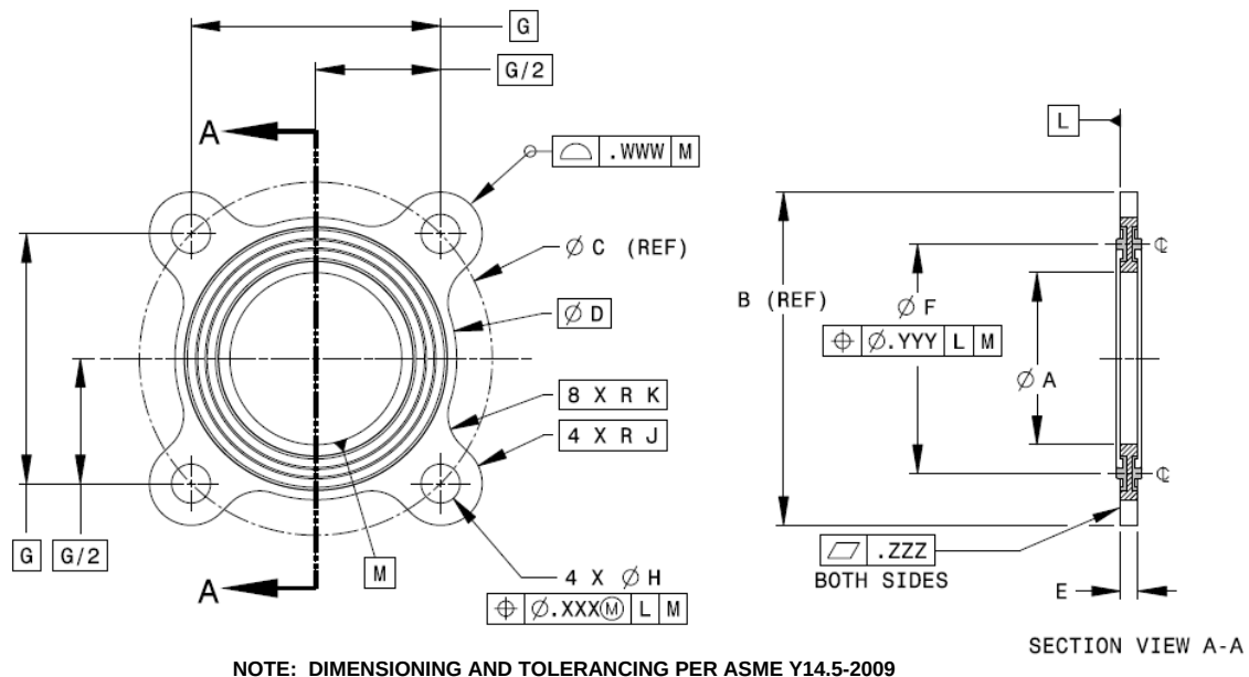
FIGURE 1 - SEAL -12 THRU -32
