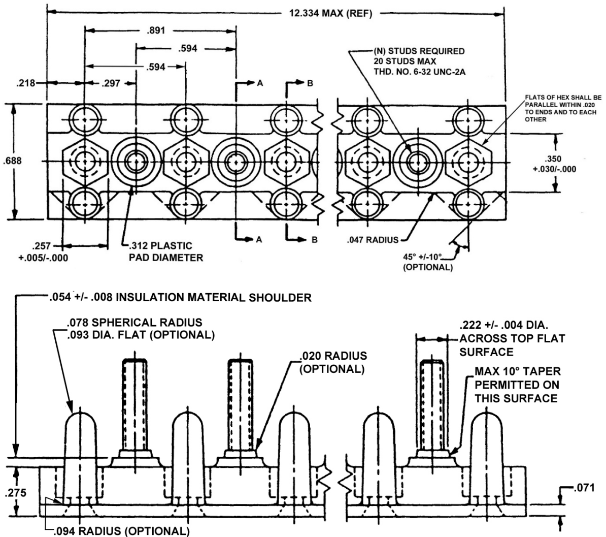
FIGURE 1 - MS27212-1-N TERMINAL BOARD
