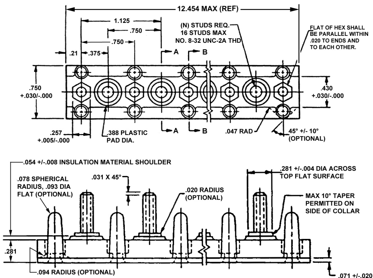
FIGURE 2 - MS27212-6-N TERMINAL BOARD
