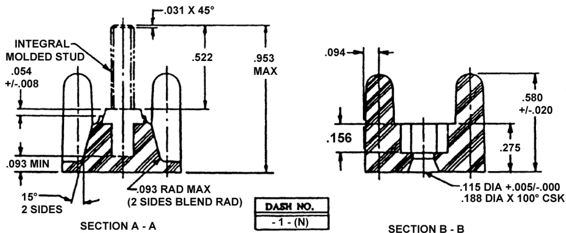
FIGURE 1 - MS27212-1-N TERMINAL BOARD (CONT.)
