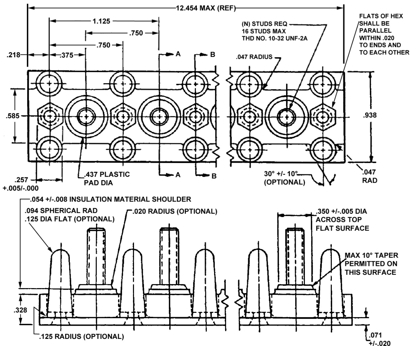
FIGURE 3 - MS27212-2-N TERMINAL BOARD
