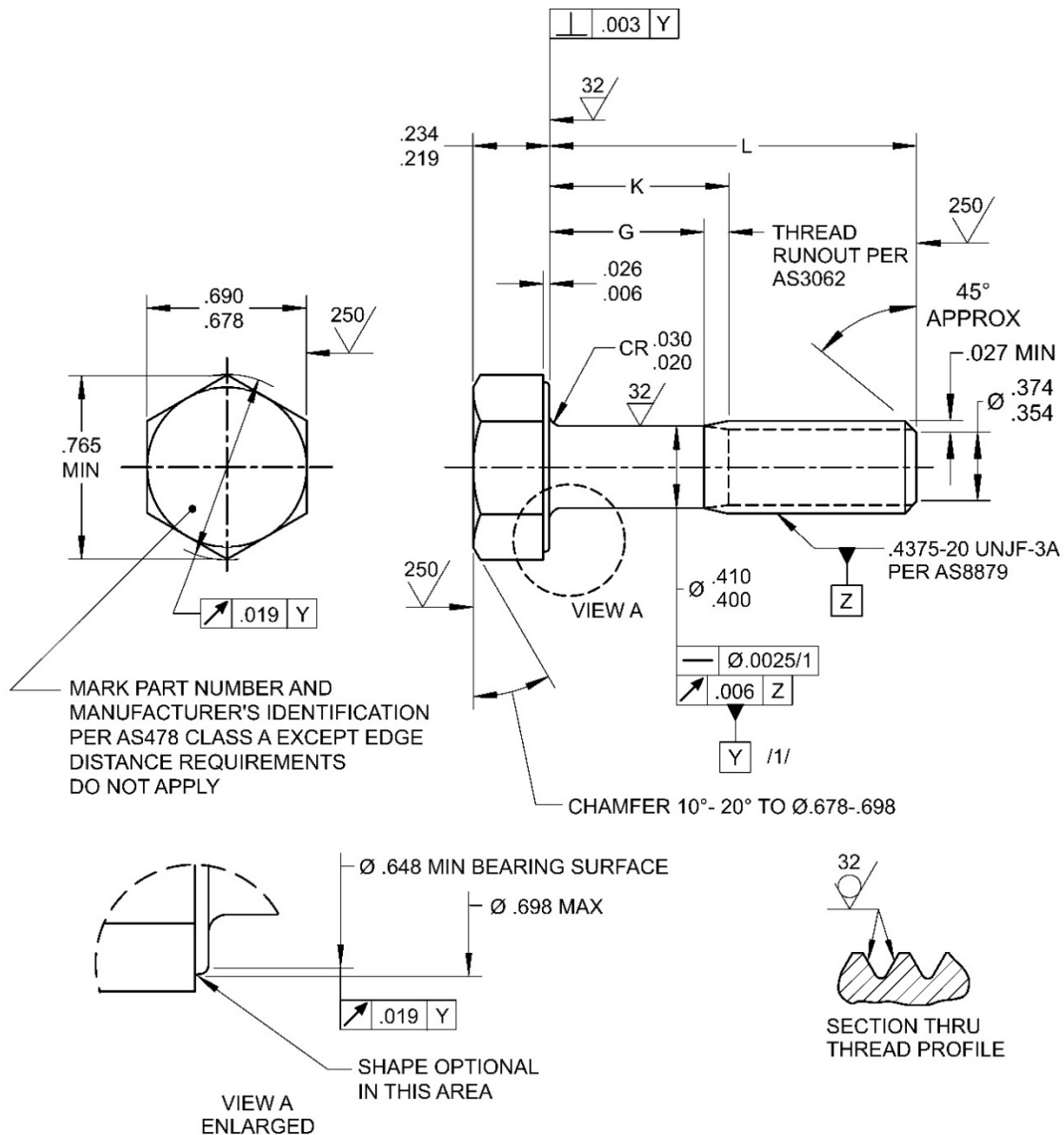
FIGURE 1 - BOLT
