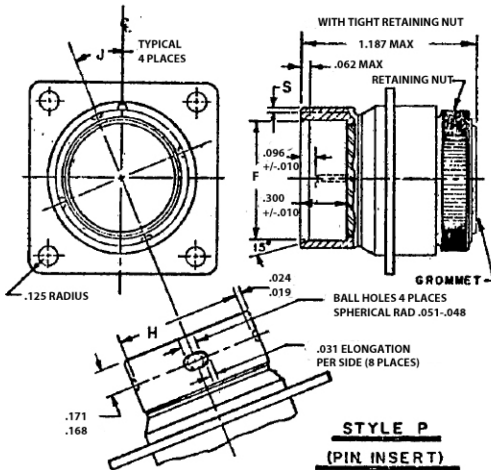
FIGURE 2 – CONNECTOR CONFIGURATIONS AND DIMENSIONS (CLASS E - CONTINUED)
