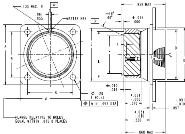
STYLE S (INSERT)
