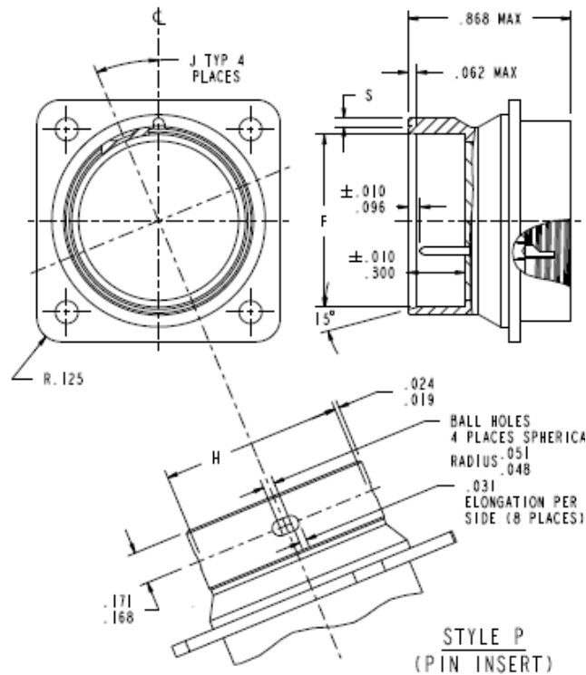
FIGURE 1 – CLASS E CONNECTOR CONFIGURATION (STYLES S AND P)
