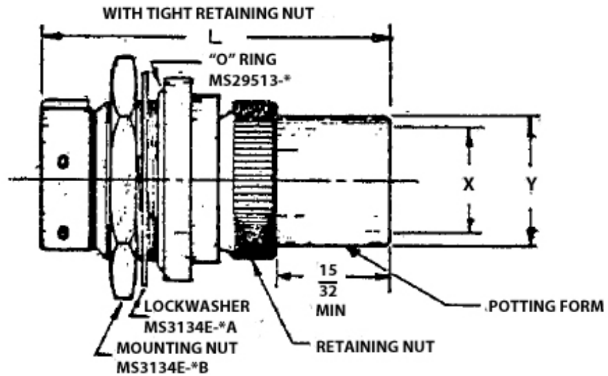
FIGURE 3 – CONNECTOR CONFIGURATIONS AND DIMENSIONS (CLASS P-POTTED SEAL)
