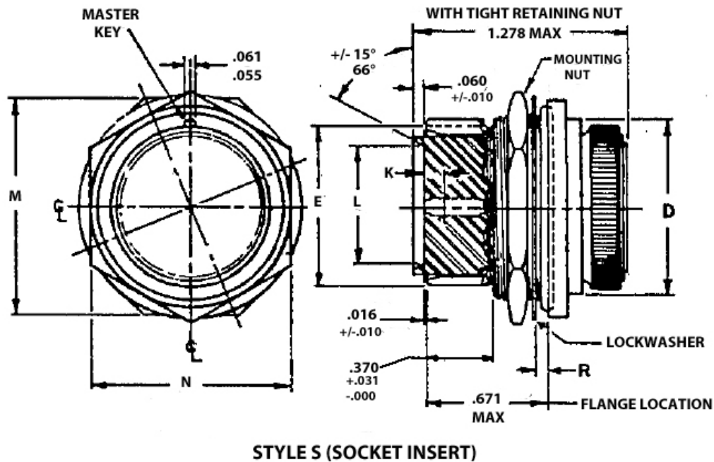
FIGURE 1 – CONNECTOR CONFIGURATIONS AND DIMENSIONS (CLASS E-STYLE S)
