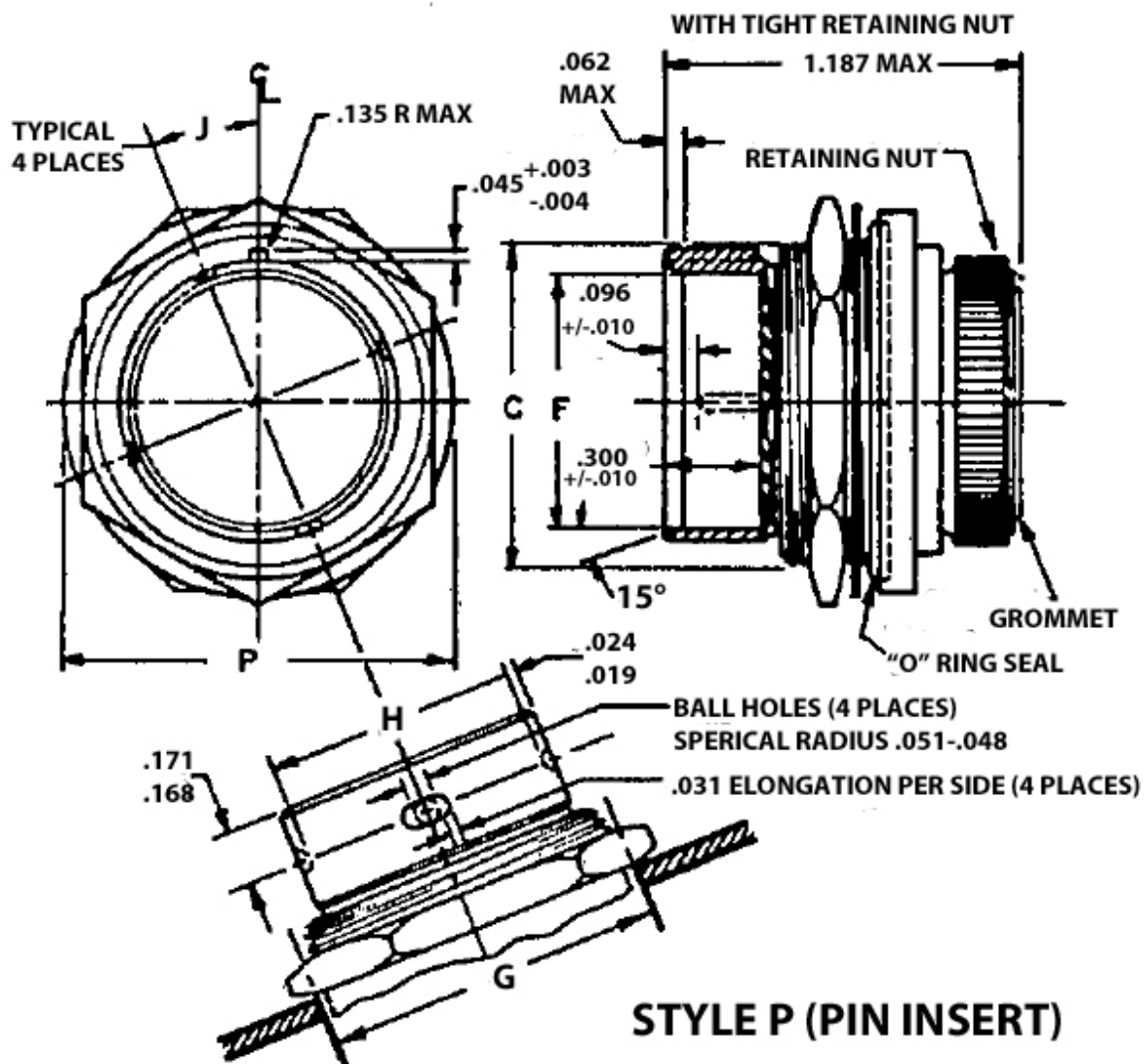
FIGURE 2 – CONNECTOR CONFIGURATIONS AND DIMENSIONS (CLASS E-STYLE P)
