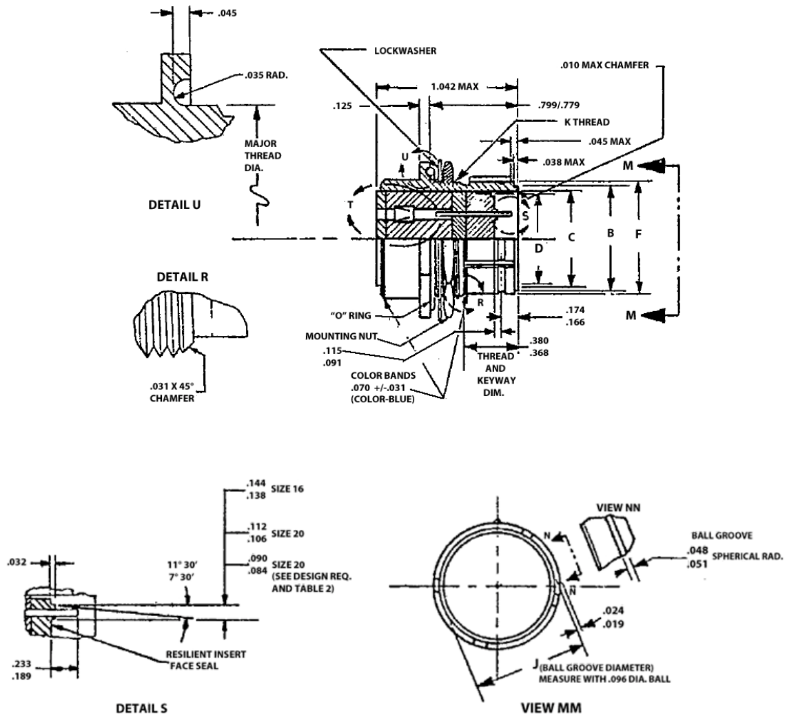
FIGURE 1 – CONNECTOR CONFIGURATIONS AND DIMENSIONS
