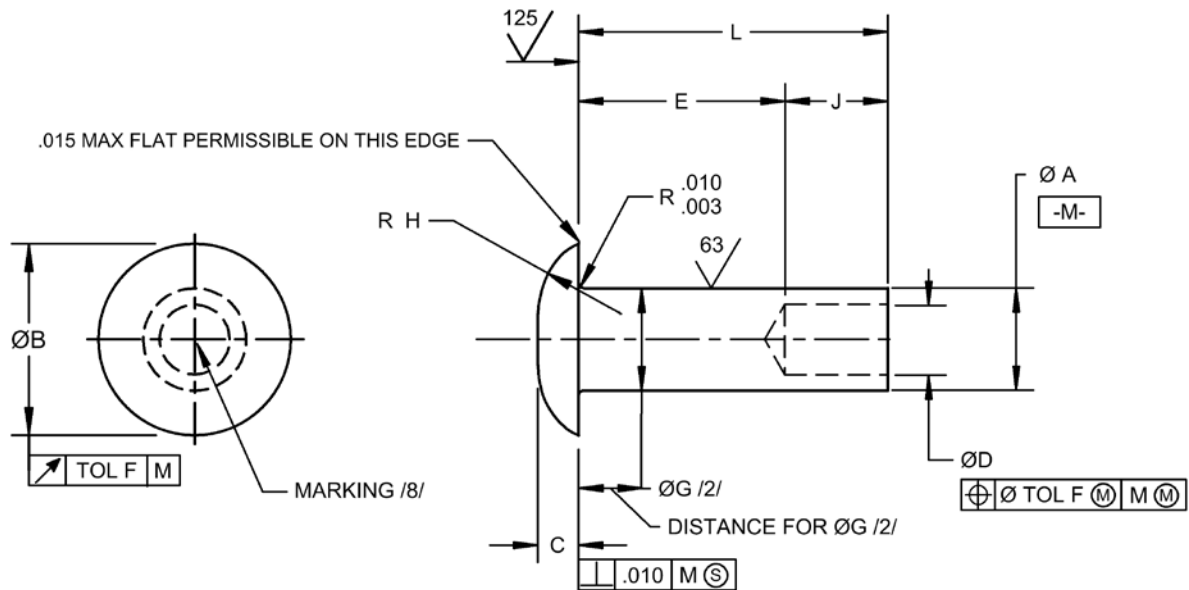
FIGURE 1 - RIVET
