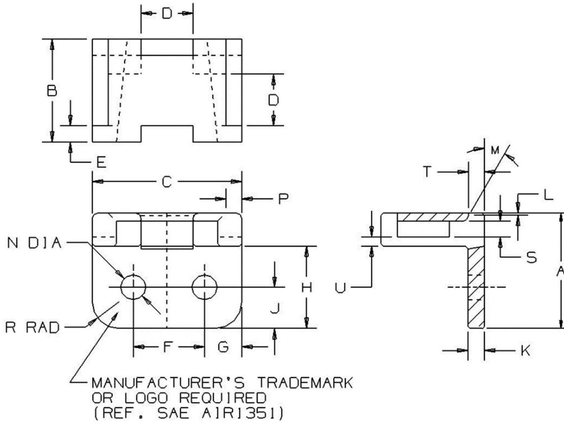
FIGURE 1 - MS3341 MOUNTING BRACKET CONFIGURATION
