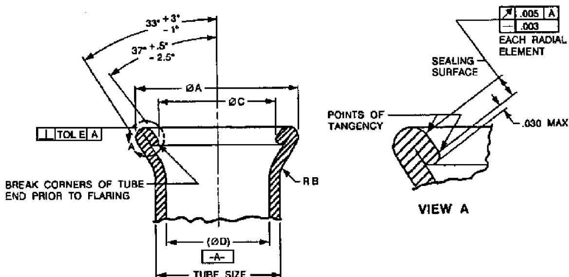
FIGURE 1 FLARED TUBE END
