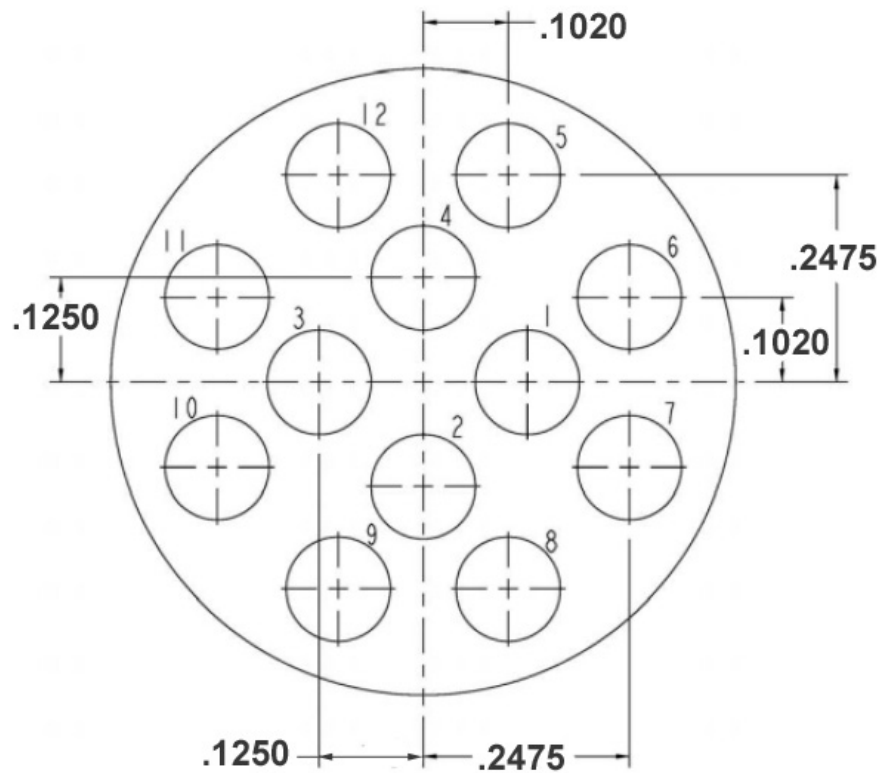
FIGURE 2 - INSERT ARRANGEMENT 19-7
