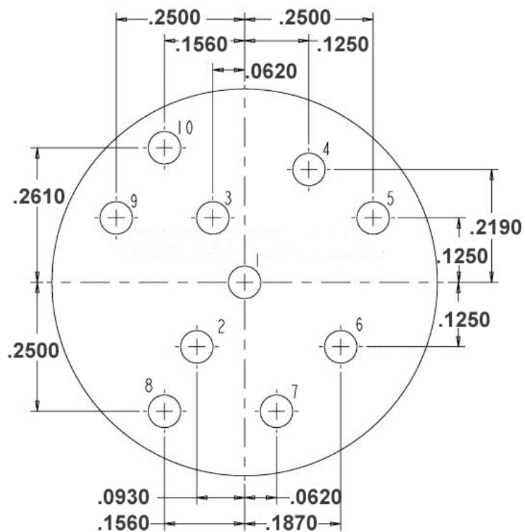
FIGURE 2 - INSERT ARRANGEMENT 27-3
