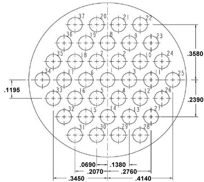
FIGURE 2 – INSERT ARRANGEMENT 37-3
