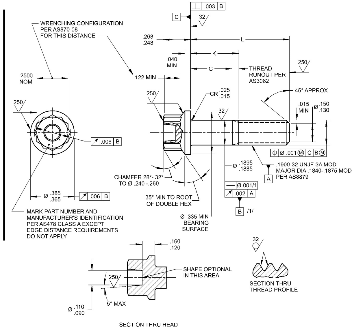
FIGURE 1 - BOLT
