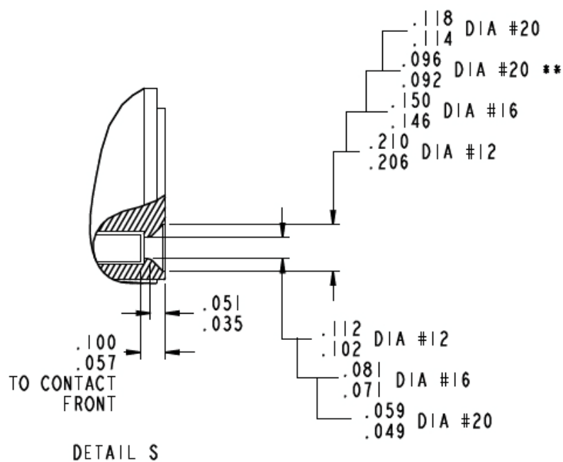
FIGURE 1B - CONNECTOR CONFIGURATION AND DIMENSIONS
