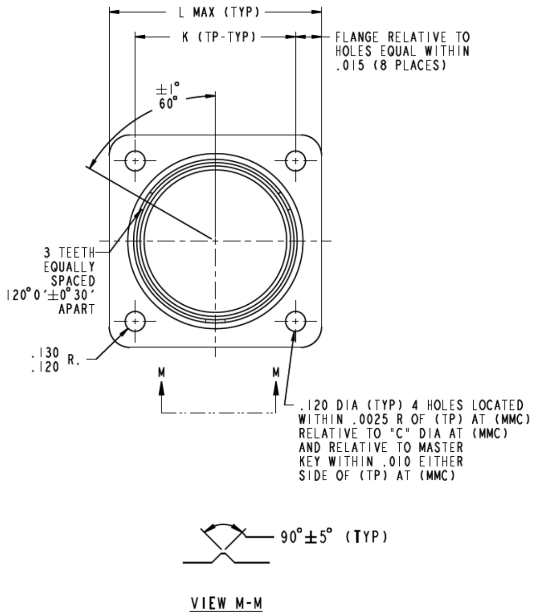
FIGURE 1A - CONNECTOR CONFIGURATION AND DIMENSIONS
