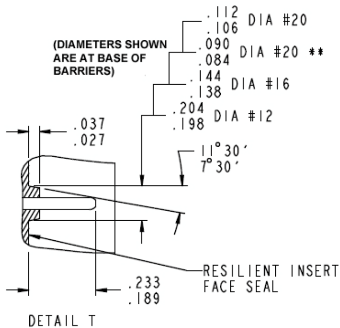
DETAIL T
