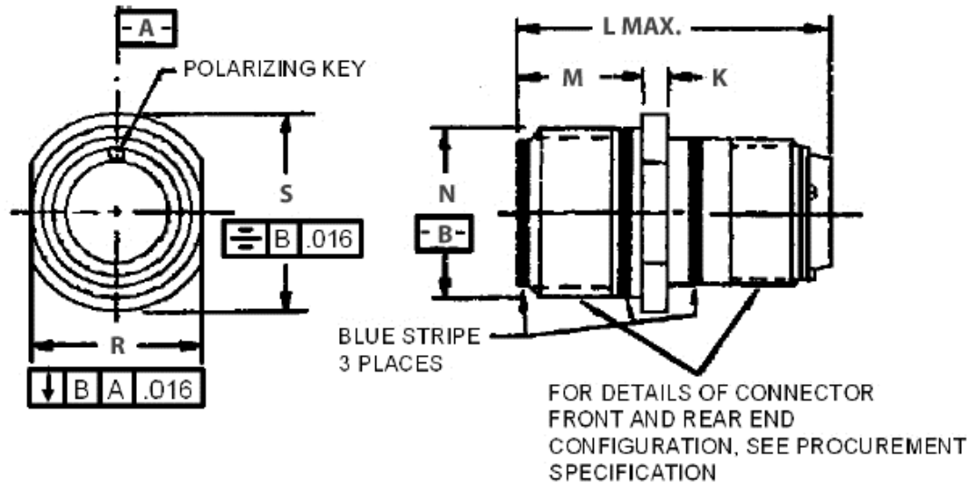
FIGURE 1 – CONNECTOR CONFIGURATION (CLASSES L,U & W ENVIRONMENT RESISTANT)
