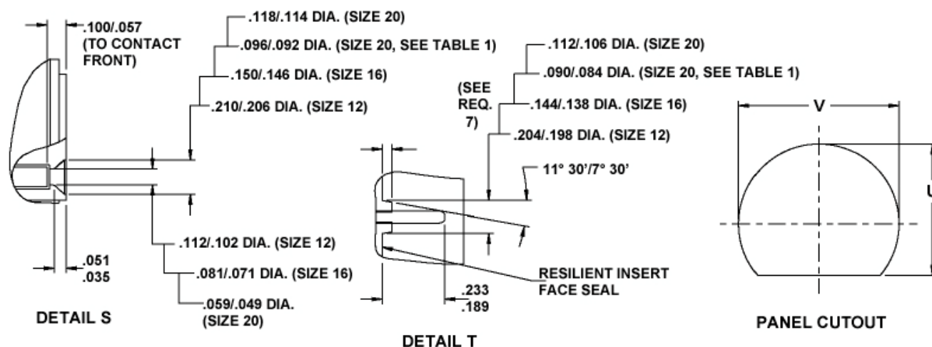
FIGURE 1 - CONNECTOR CONFIGURATIONS AND DIMENSIONS (CONTINUED)
