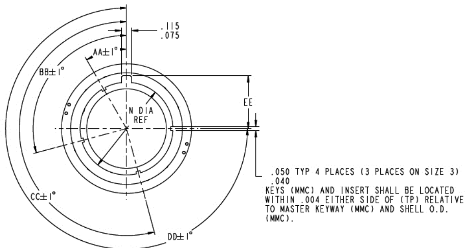
FIGURE 3 - CONNECTOR KEY POSITIONS
