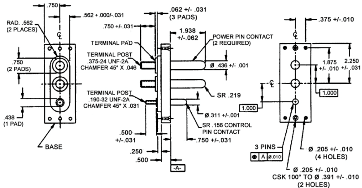
FIGURE 2 - BASE AND CONTACT ASSEMBLY
