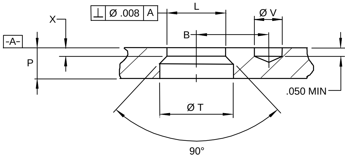
FIGURE 2 - INSTALLATION HOLE
