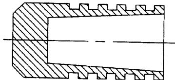
FIGURE 2 - AS3127 PLUG
