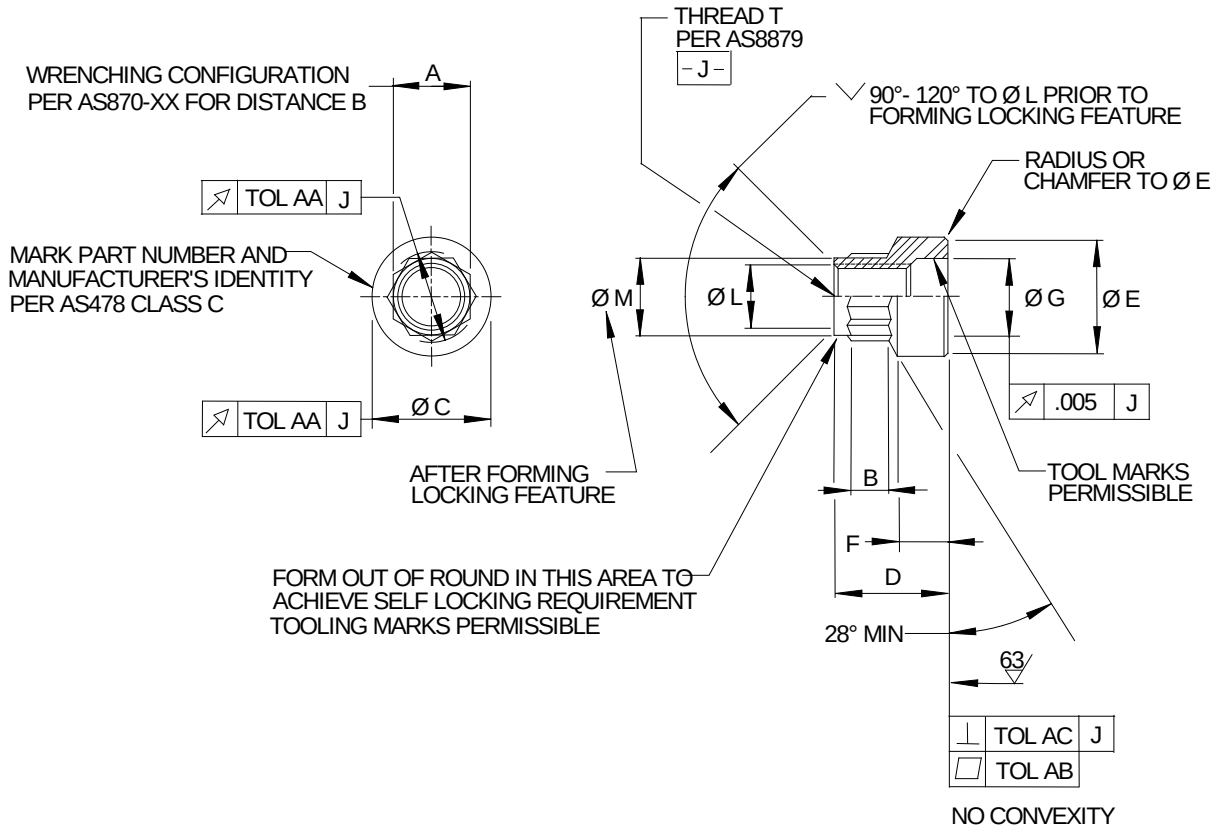
FIGURE 1 - NUT
