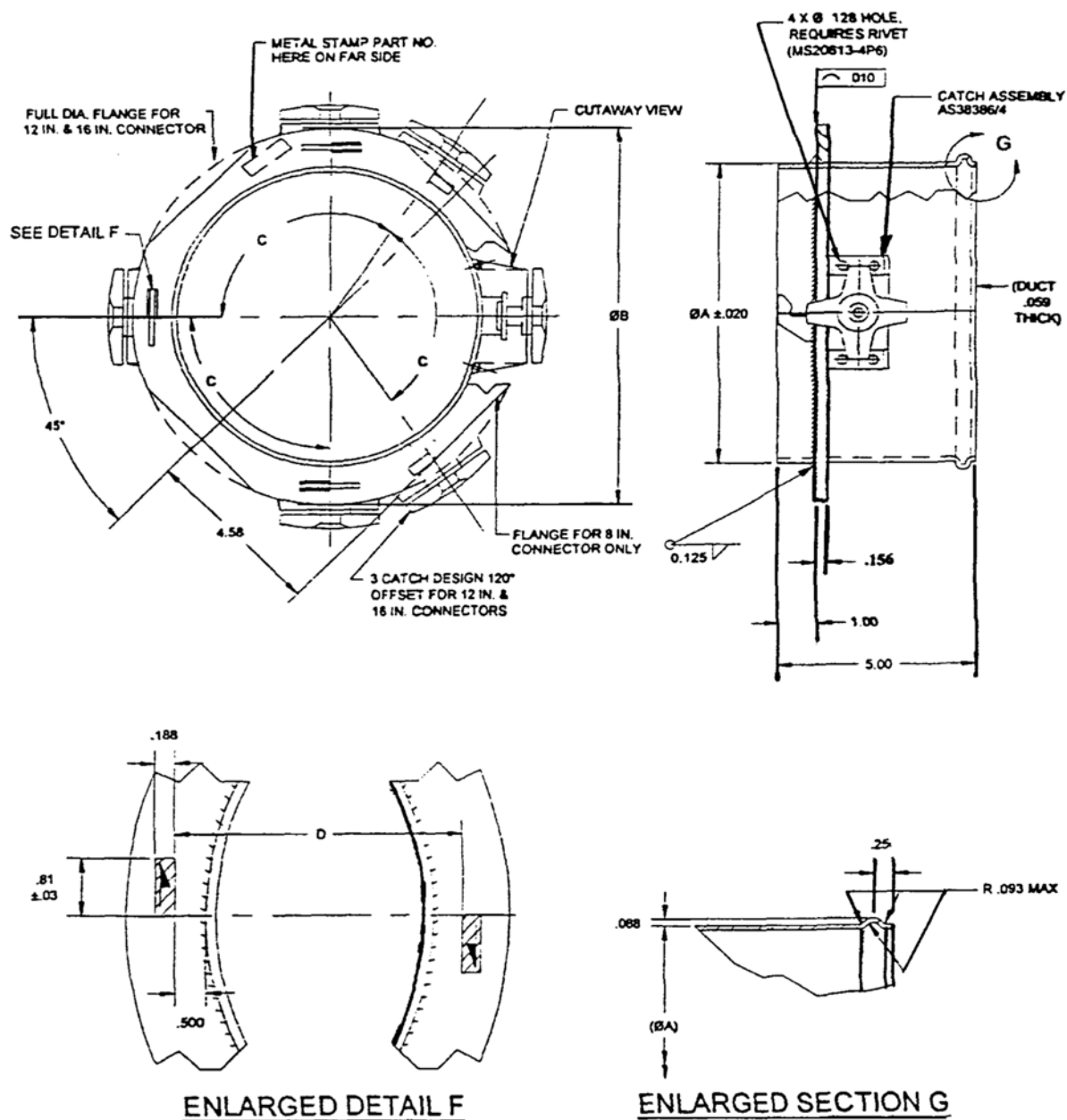
FIGURE 1 - MALE CONNECTOR
