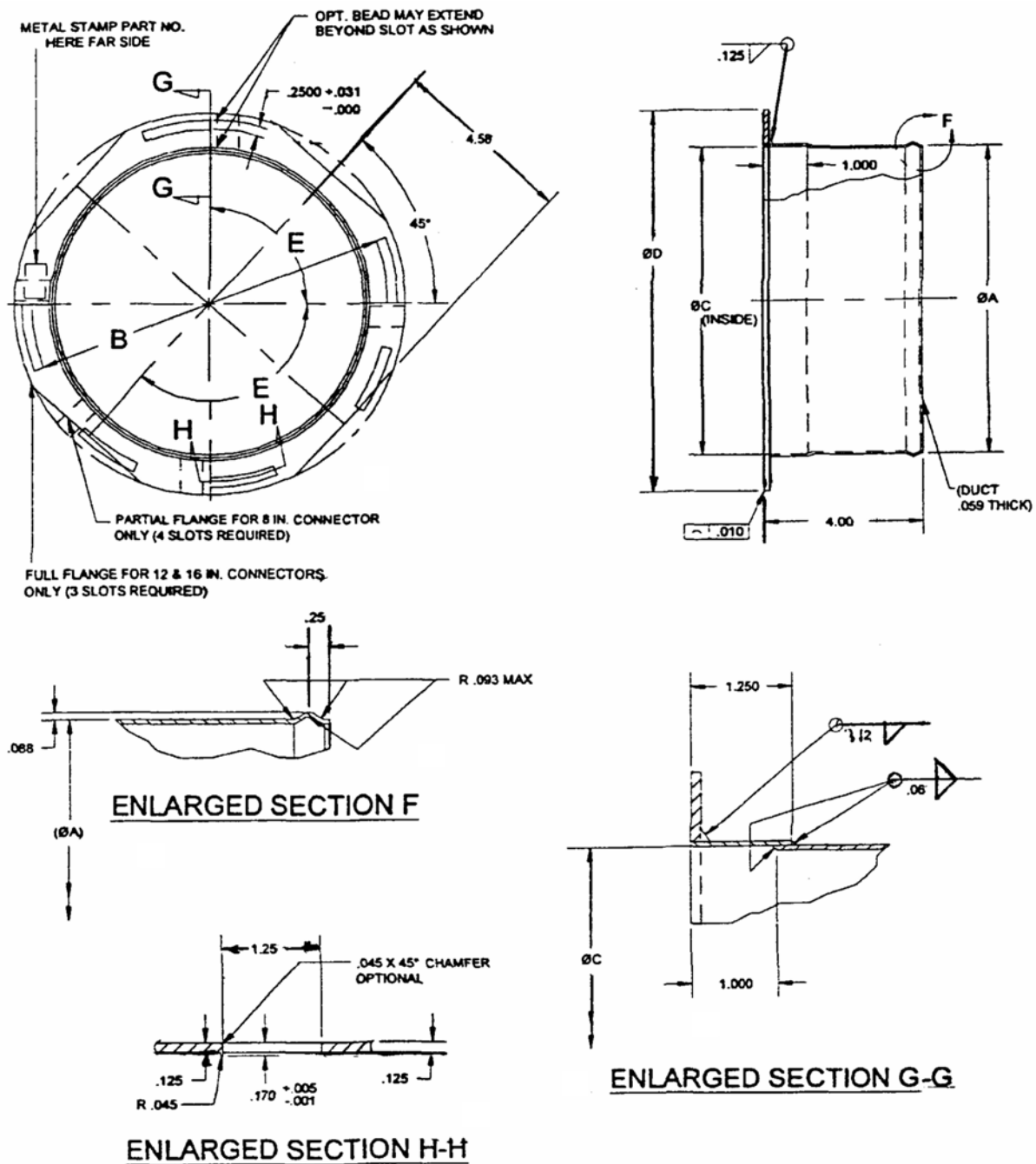
FIGURE 1 - FEMALE CONNECTOR
