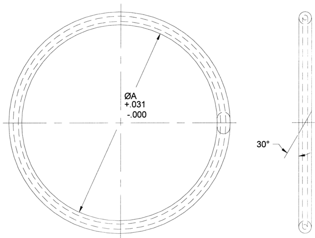
FIGURE 1 - PREFORMED PACKING
