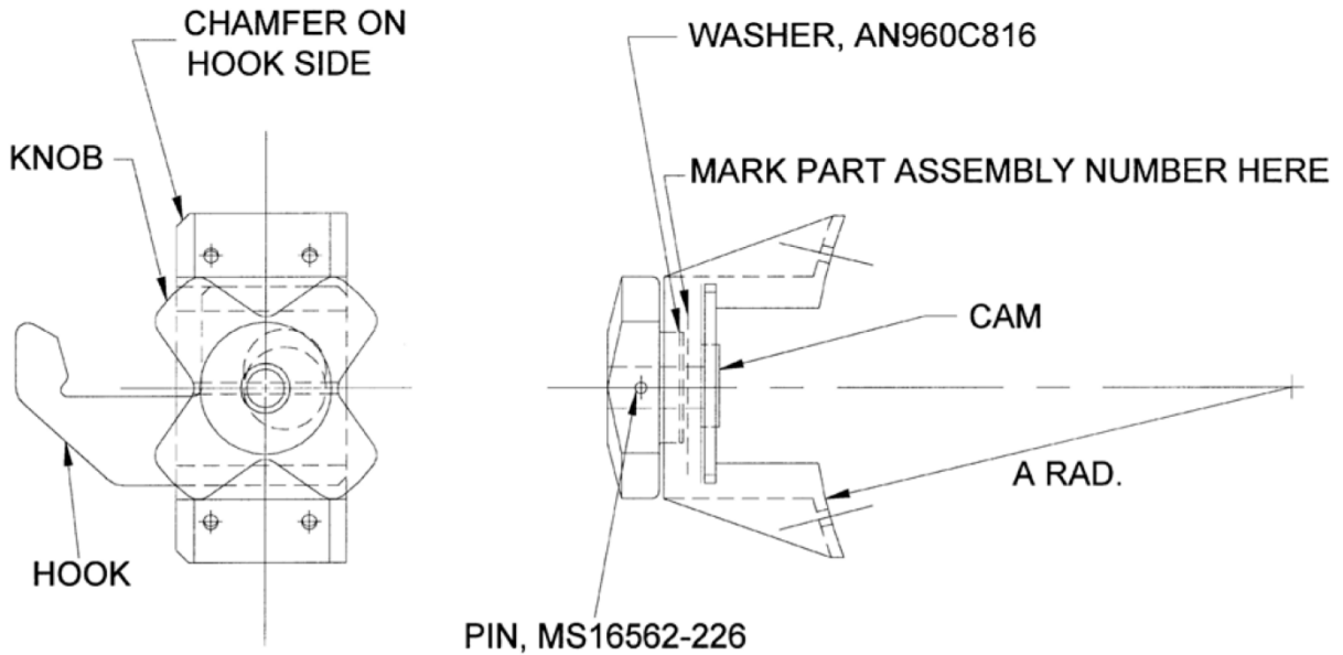
FIGURE 1 - CATCH ASSEMBLY
