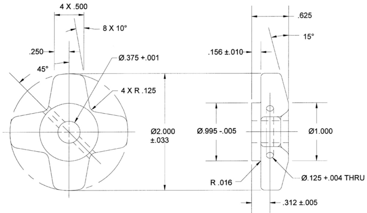
FIGURE 2 - KNOB
