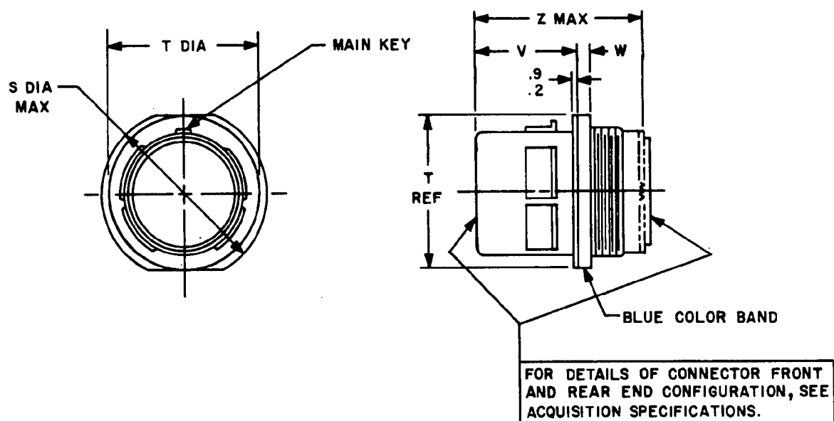
FIGURE 1. RECEPTACLE, CLASSES C, F AND W
