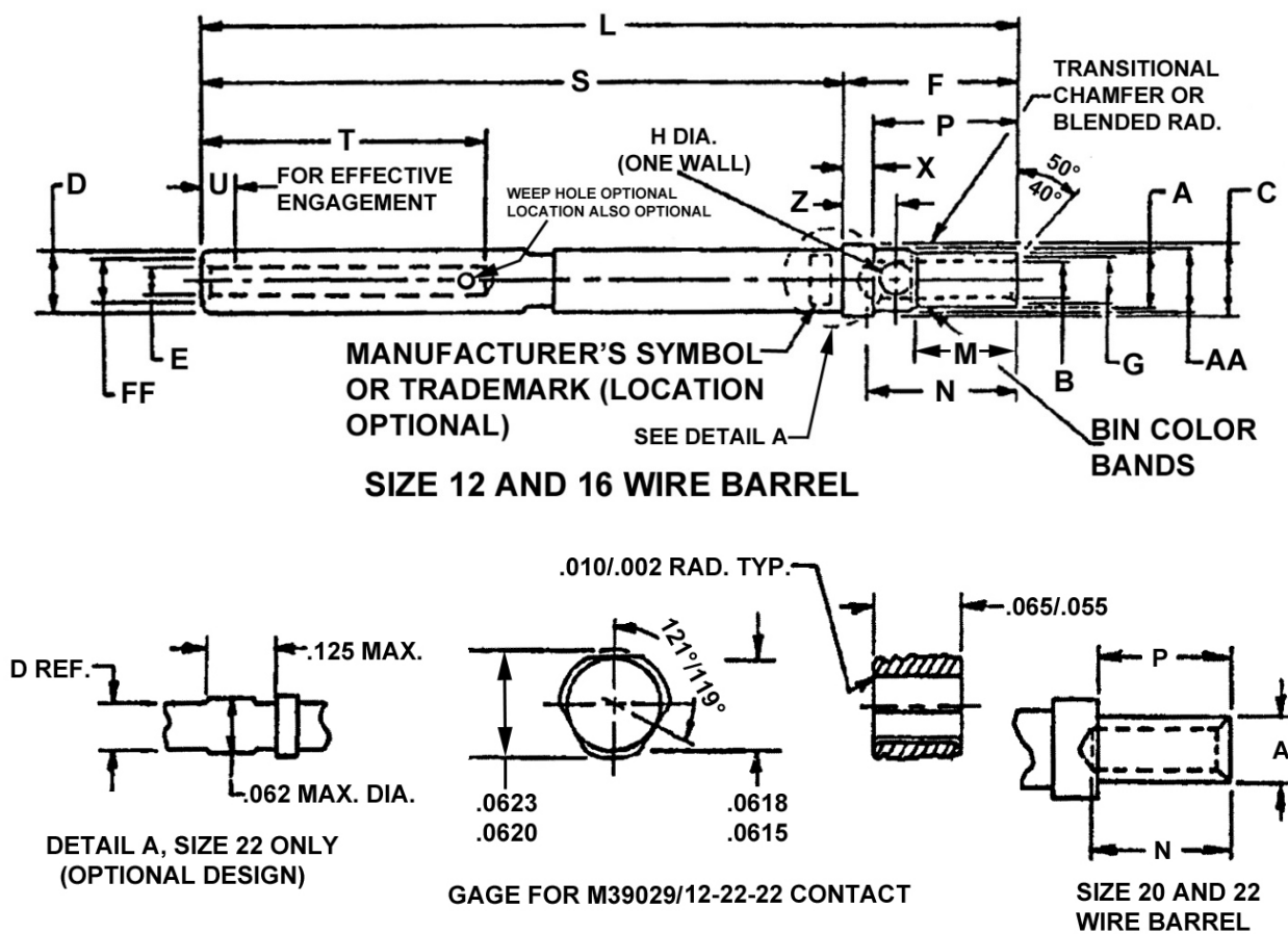
FIGURE 1 - SOCKET CONTACT
