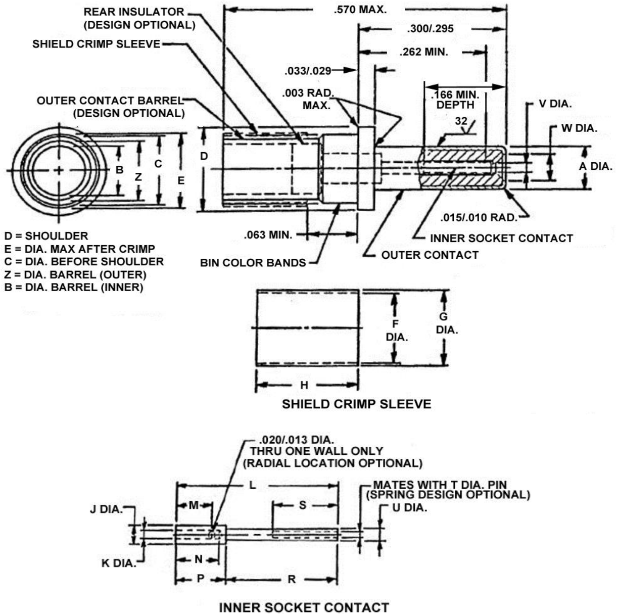
FIGURE 1 - PIN CONTACTS
